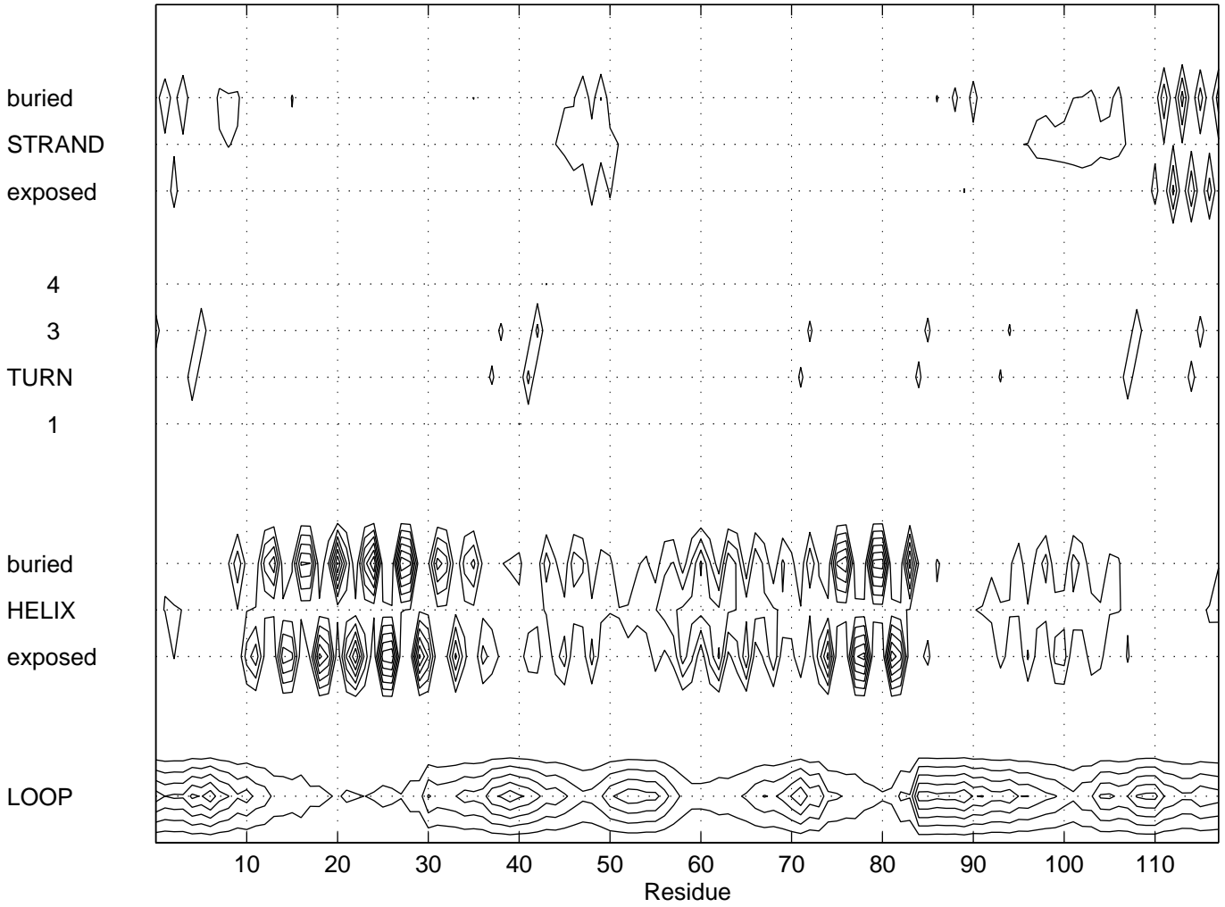
Secondary-structure probabilities for Sequence 23 (vsp7.m)
