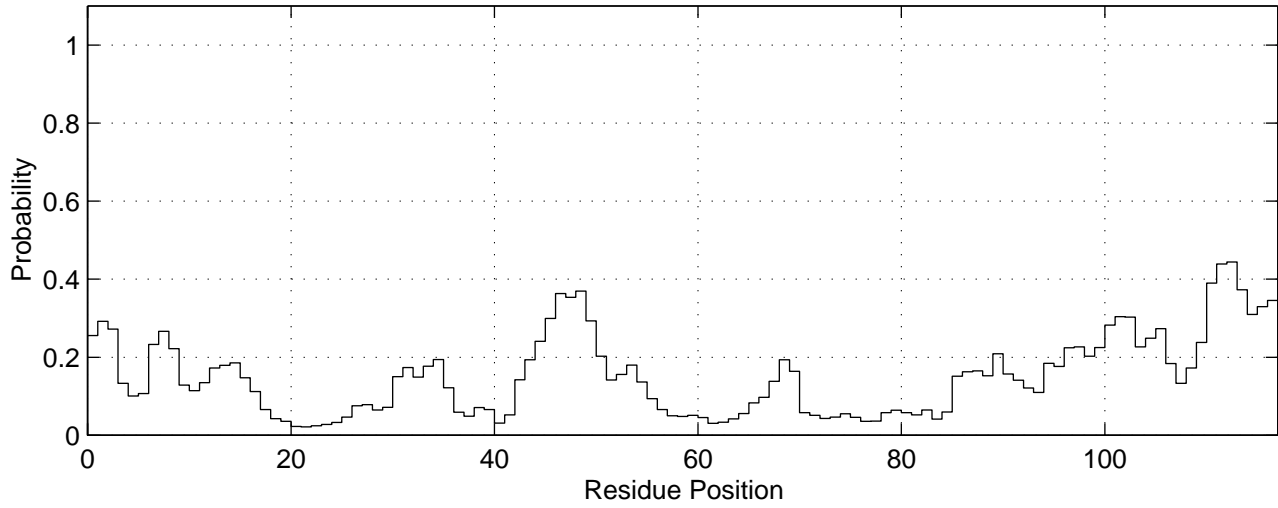
Probability of being in a turn for Sequence 23 (psp3.m), 18-Nov-98 (17:57:56)
