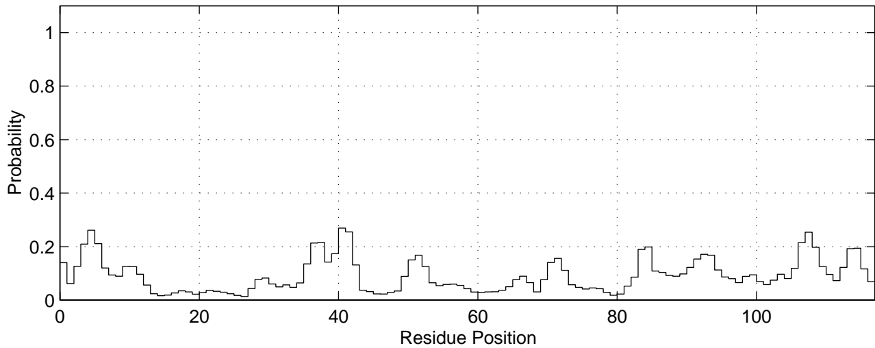
Probability of being in a helix for Sequence 23 (psp3.m), 18-Nov-98 (17:57:57)
