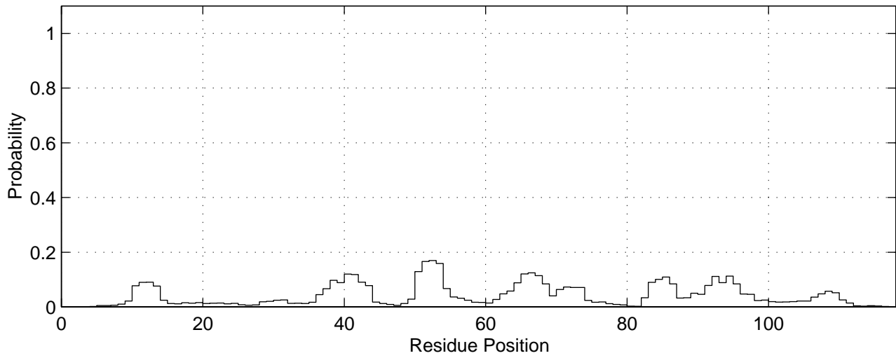
Probability of being in a helix for Sequence 23 (psp3.m), 18-Nov-98 (17:52:51)
