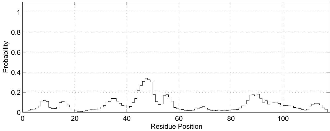
Probability of being in a turn for Sequence 23 (psp3.m), 18-Nov-98 (17:52:50)
